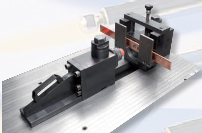
BUS BARS punching Poansonat de bare de cupru
