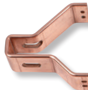
Copper bus-bar punched and bent Electric cabinets
